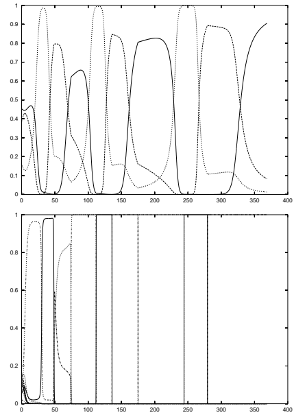
Figure 2: An example of dynamics of RED with the inverse standard deviation type meta-rule (Eq.(7)). The y axes are the strategy distribution for the top graph and the weights of games for the bottom, respectively. The x axis is time steps. The system size is N = 3, M = 10 .
